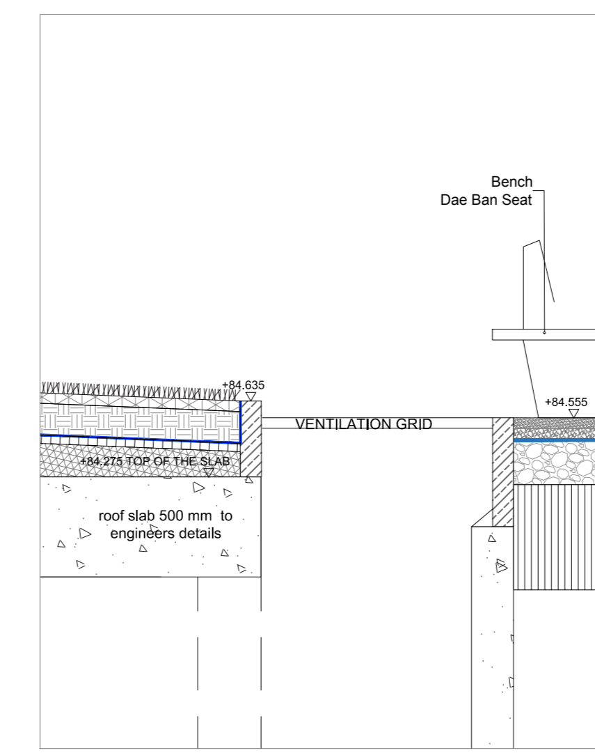
DETAIL 1C DETAIL SECTION CC VENT EDGE, SCALE 1:25@A0
