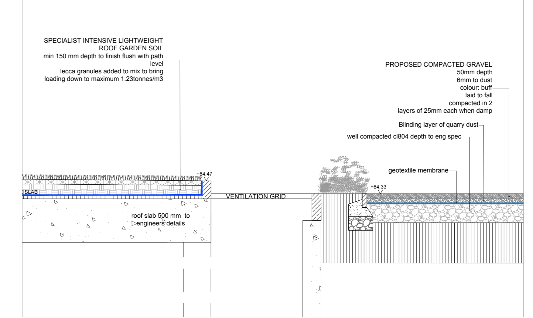
DETAIL 2D DETAIL SECTION HH: VENT/PLANTER EDGE, SCALE 1:25@A0
