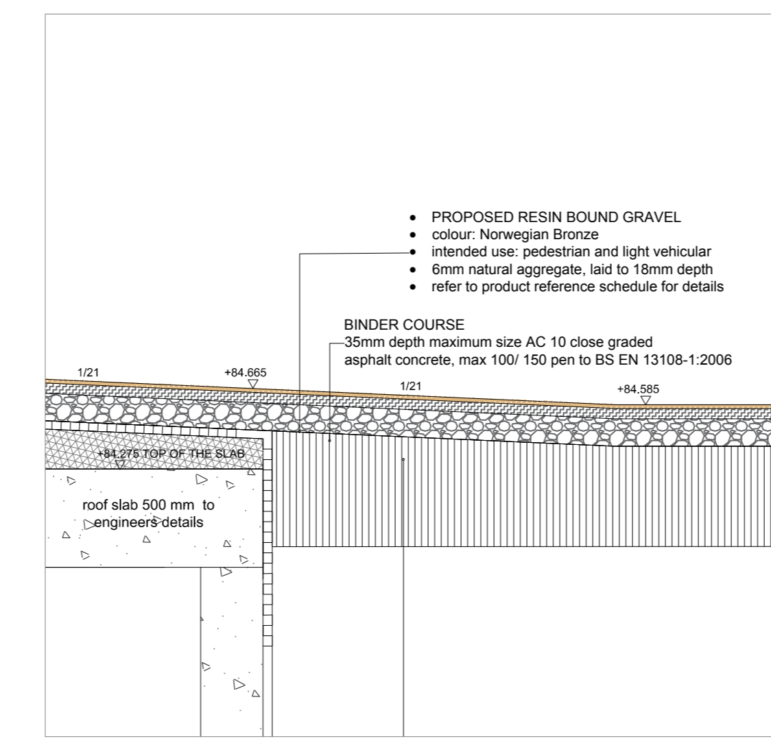
DETAIL 1B DETAIL SECTION BB PATH DETAIL, SCALE 1:25@A0
