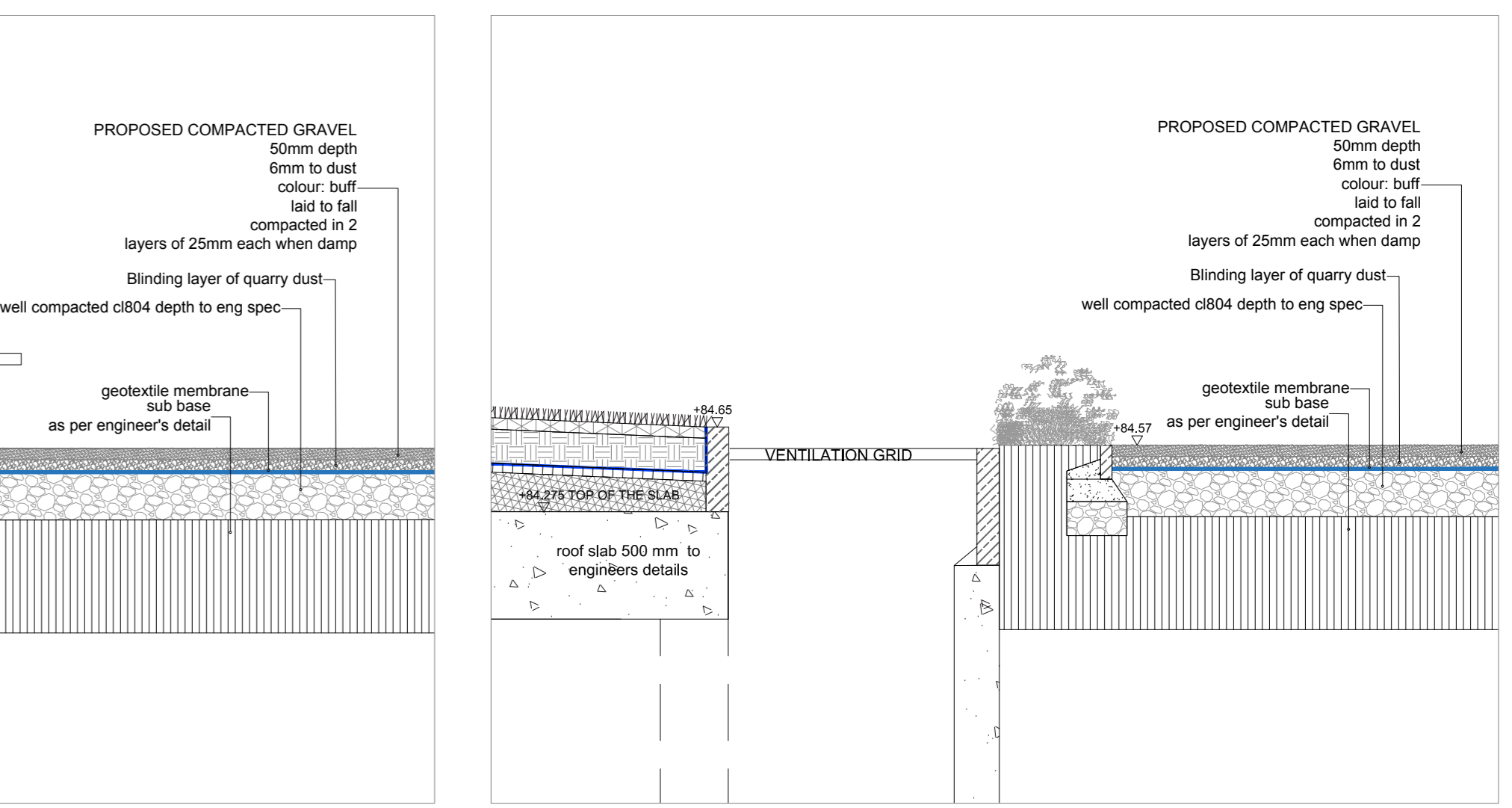
DETAIL 1D DETAIL SECTION DD: VENT/PLANTER EDGE, SCALE 1:25@A0
