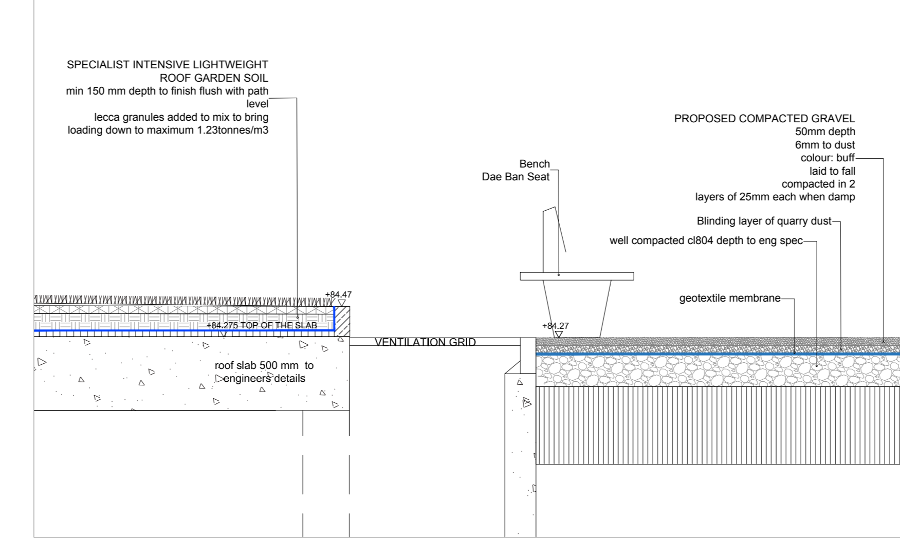
DETAIL 2C DETAIL SECTION GG VENT EDGE, SCALE 1:25@A0
